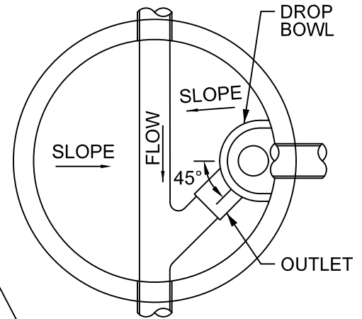
INSIDE DROP PLAN VIEW NOT TO SCALE
