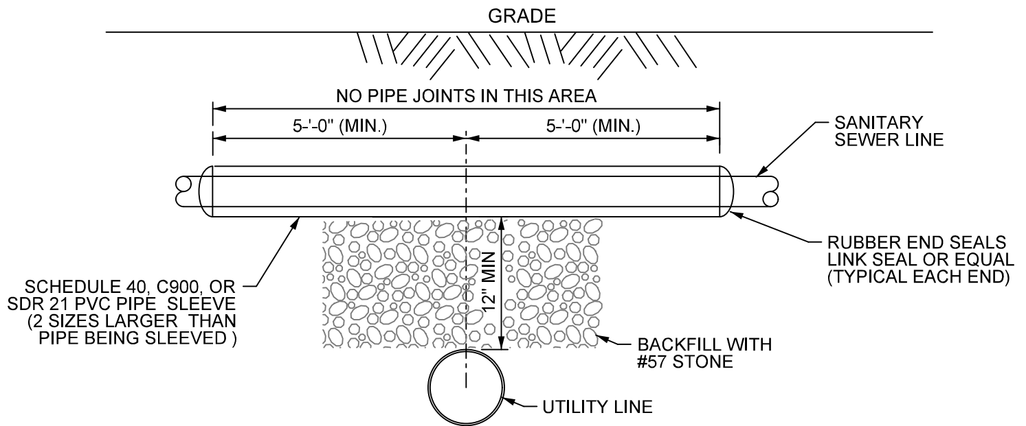
TYPICAL SEWER OVER UTILITY LINE CROSSING
