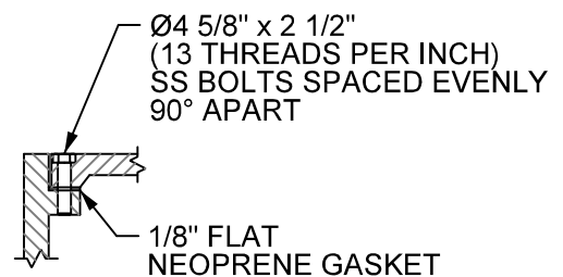
WATERTIGHT DETAIL
